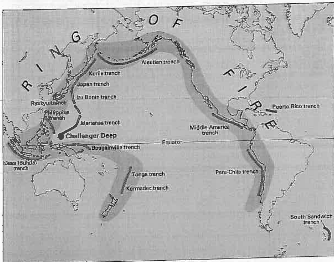
Ring of Fire (URL: pubs.usgs.gov/publications/text/fire.html )
