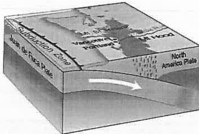
Cascadia Subduction Zone under British Columbia, Washington and Oregon (Source: USGS)
